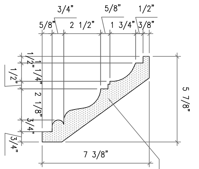
CORNICE DETAIL 03
