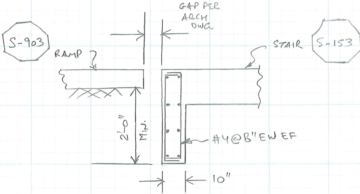
SECTION X 1
