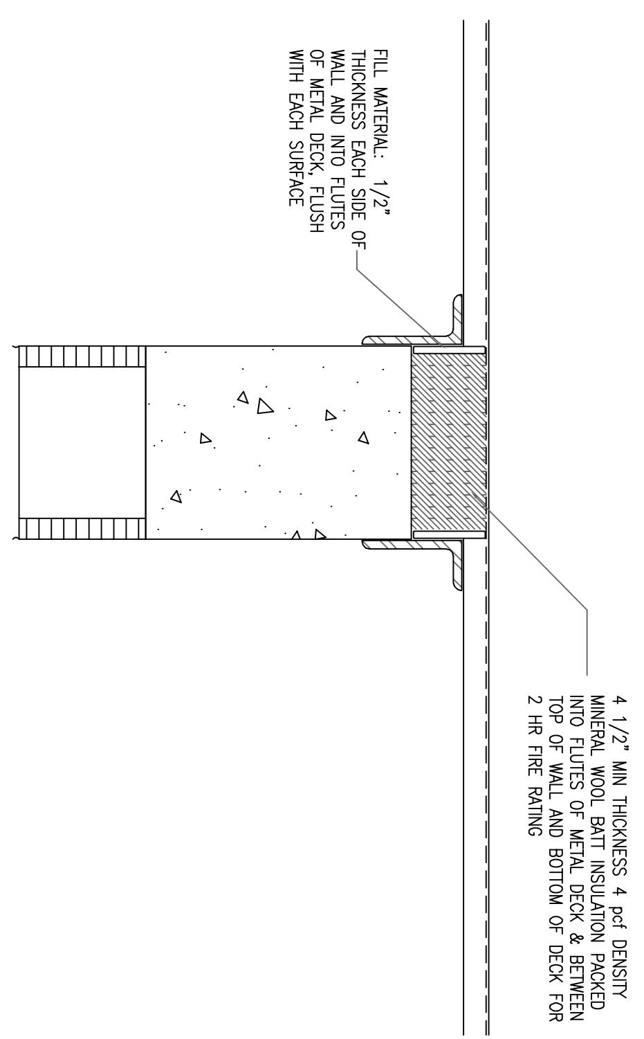
WALL TO ROOF DETAIL 05
